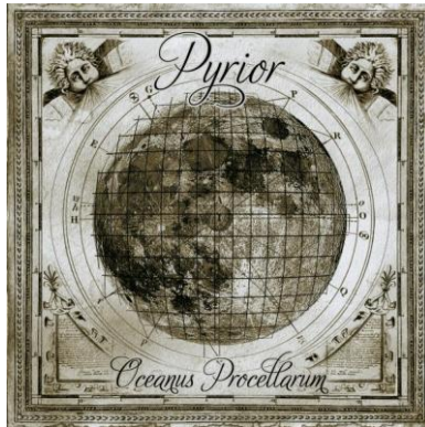
Oceanus Procellarum LP (2010)
